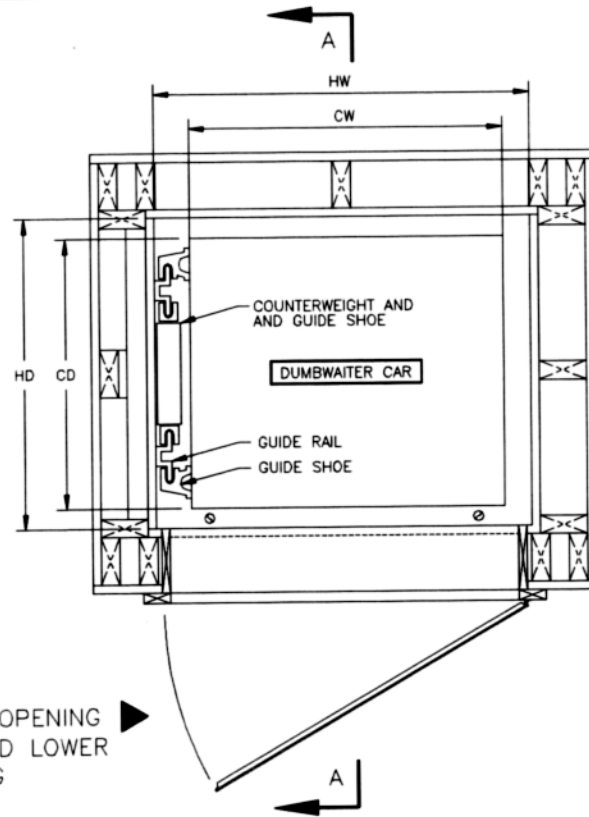
PLAN VIEW TYPICAL WOOD FRAMING
